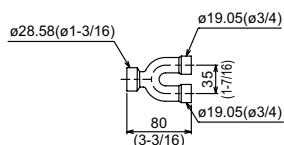
High-pressure twinning pipe
