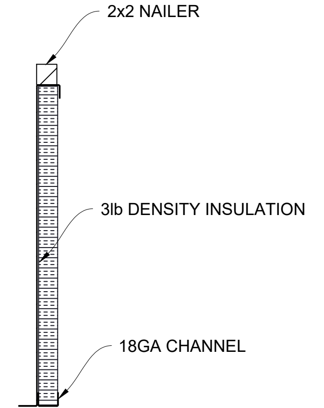
DETAIL A
